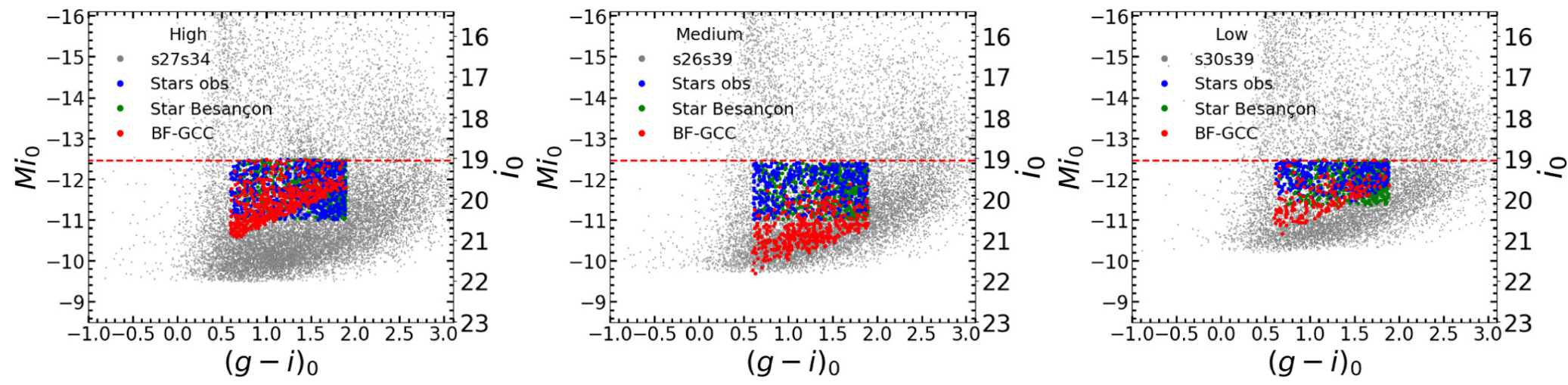
Figure 9. from Luis Lomelí-Núñez et al 2025 Astron. J. 169 doi:10.3847/1538-3881/adbf0c https://dx.doi.org/10.3847/1538-3881/adbf0c © 2025. The Author(s). Published by the American Astronomical Society.
