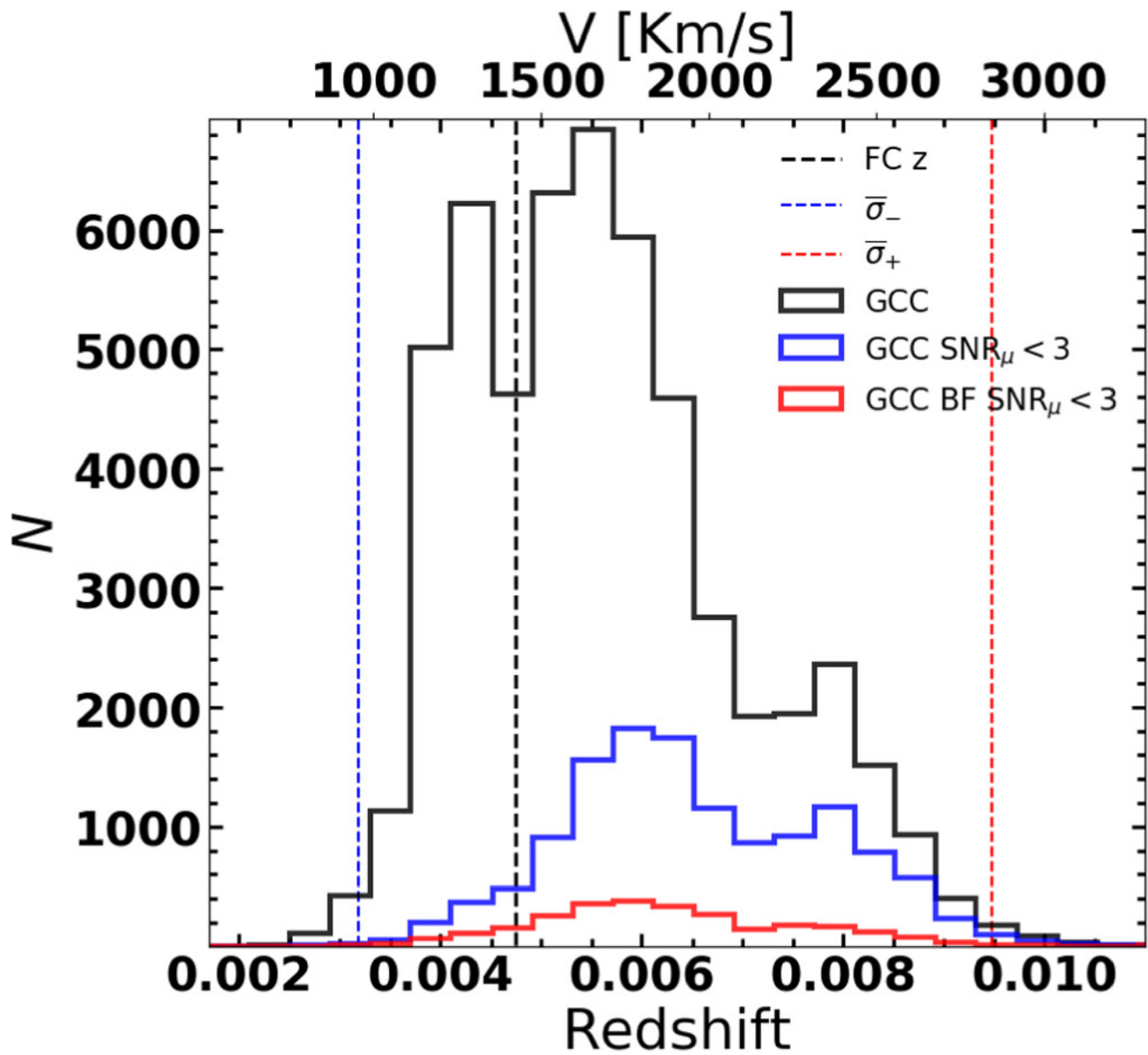
Figure 8. from Luis Lomelí-Núñez et al 2025 Astron. J. 169 doi:10.3847/1538-3881/adbf0c https://dx.doi.org/10.3847/1538-3881/adbf0c © 2025. The Author(s). Published by the American Astronomical Society.
