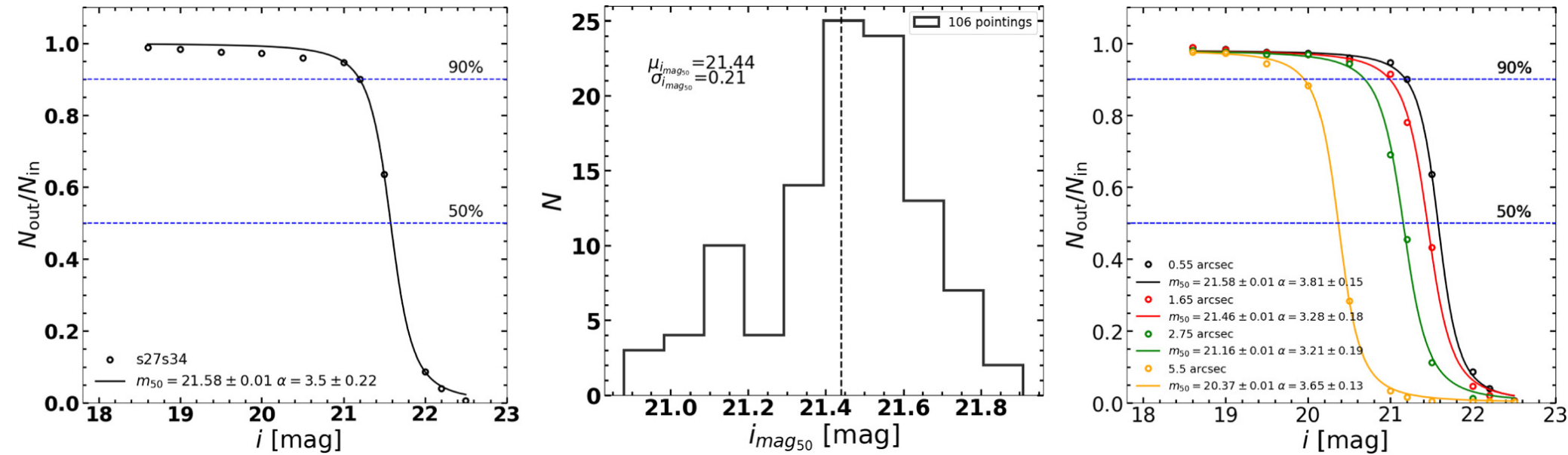
Figure 5. from Luis Lomelí-Núñez et al 2025 Astron. J. 169 doi:10.3847/1538-3881/adbf0c https://dx.doi.org/10.3847/1538-3881/adbf0c © 2025. The Author(s). Published by the American Astronomical Society.
