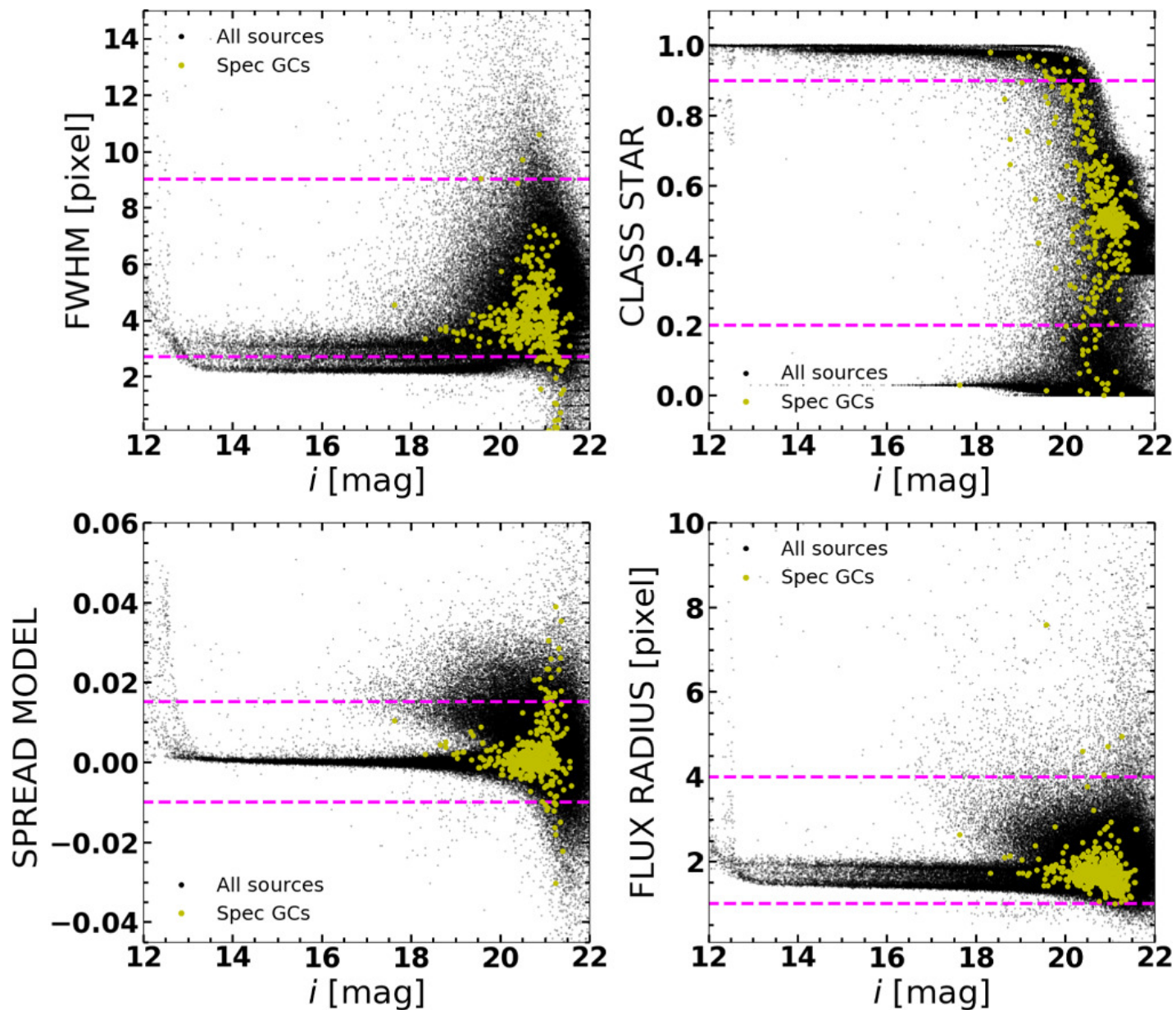
Figure 4. from Luis Lomelí-Núñez et al 2025 Astron. J. 169 doi:10.3847/1538-3881/adbf0c https://dx.doi.org/10.3847/1538-3881/adbf0c © 2025. The Author(s). Published by the American Astronomical Society.
