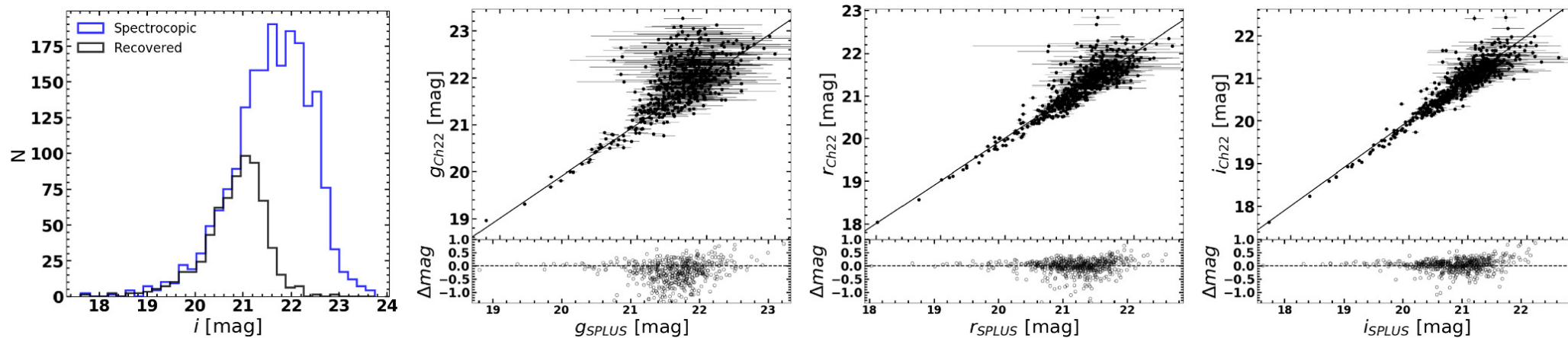
Figure 3. from Luis Lomelí-Núñez et al 2025 Astron. J. 169 doi:10.3847/1538-3881/adbf0c https://dx.doi.org/10.3847/1538-3881/adbf0c © 2025. The Author(s). Published by the American Astronomical Society.
