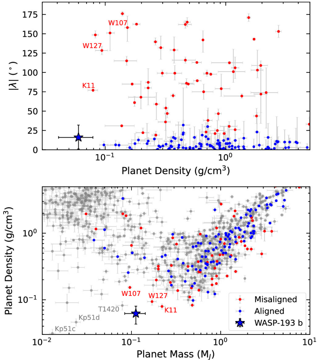
Figure 6. from Samuel W. Yee et al 2025 Astron. J. 169 doi:10.3847/1538-3881/adba5f https://dx.doi.org/10.3847/1538-3881/adba5f © 2025. The Author(s). Published by the American Astronomical Society.
