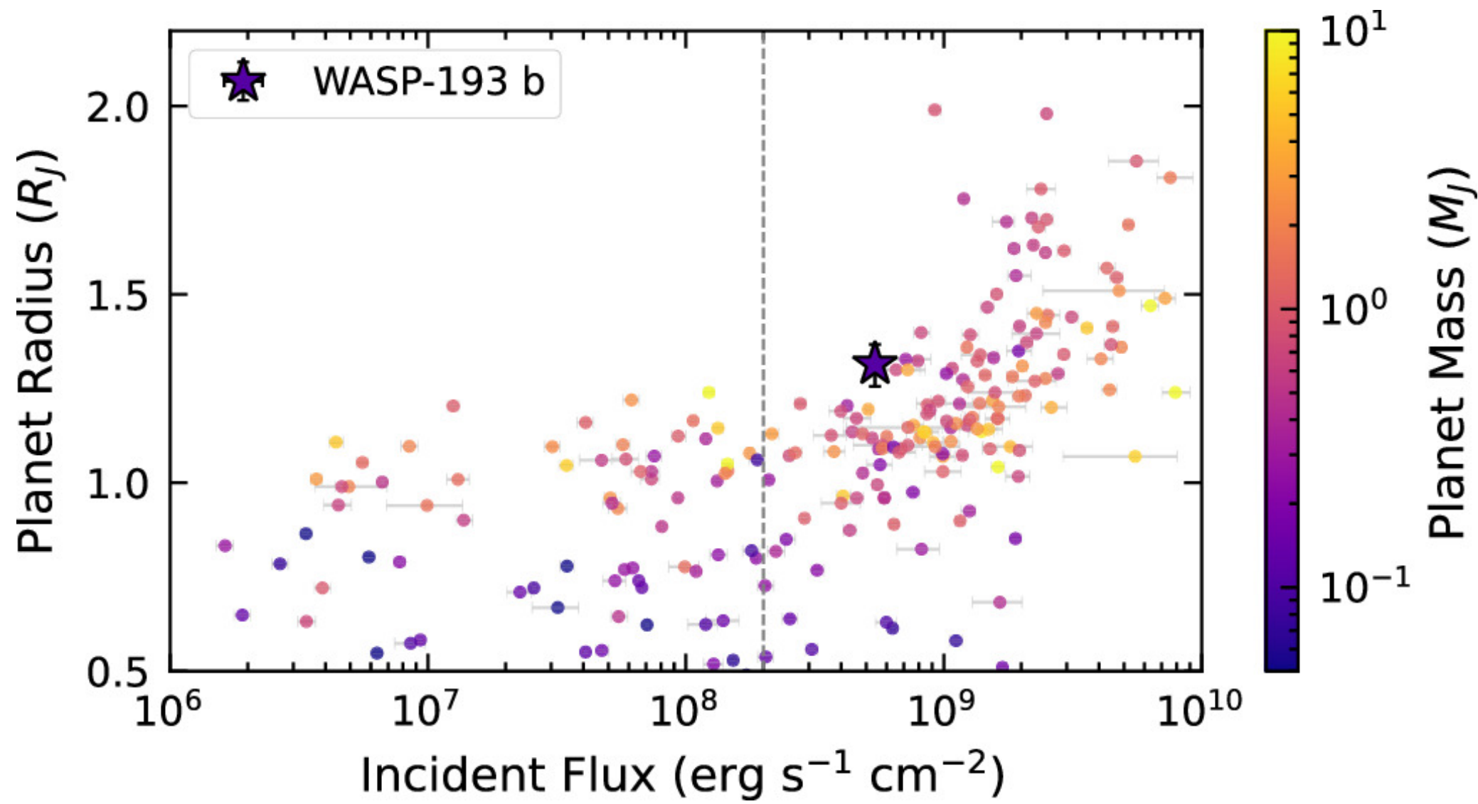
Figure 5. from Samuel W. Yee et al 2025 Astron. J. 169 doi:10.3847/1538-3881/adba5f https://dx.doi.org/10.3847/1538-3881/adba5f © 2025. The Author(s). Published by the American Astronomical Society.
