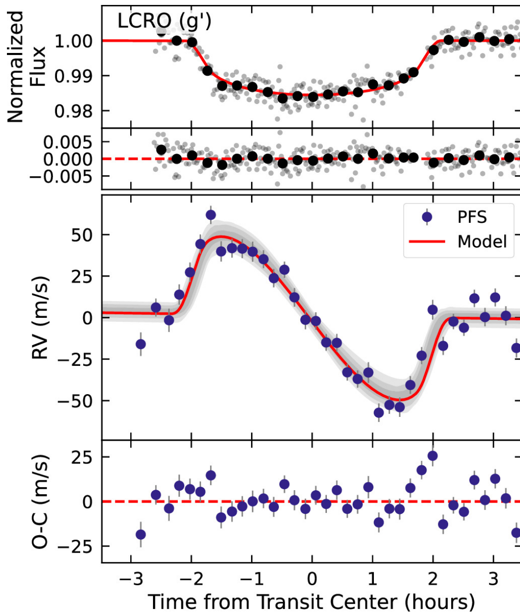
Figure 4. from Samuel W. Yee et al 2025 Astron. J. 169 doi:10.3847/1538-3881/adba5f https://dx.doi.org/10.3847/1538-3881/adba5f © 2025. The Author(s). Published by the American Astronomical Society.
