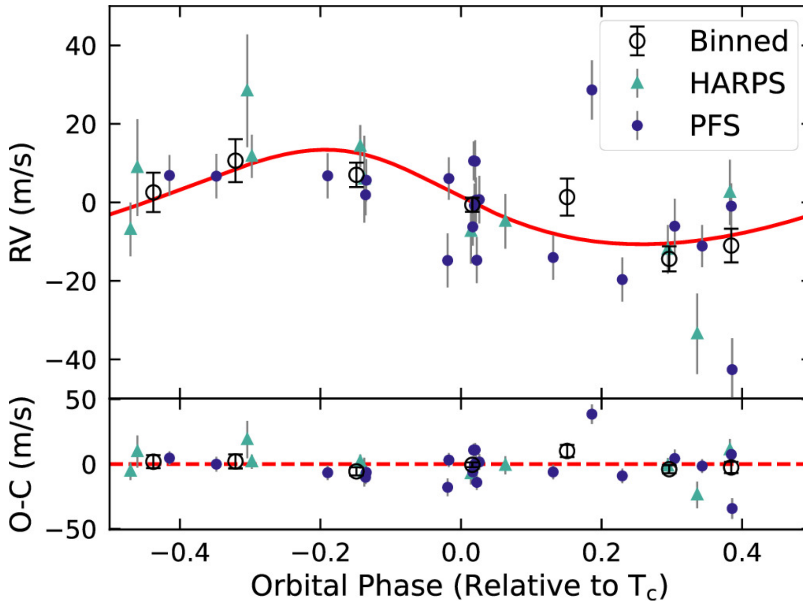
Figure 3. from Samuel W. Yee et al 2025 Astron. J. 169 doi:10.3847/1538-3881/adba5f https://dx.doi.org/10.3847/1538-3881/adba5f © 2025. The Author(s). Published by the American Astronomical Society.
