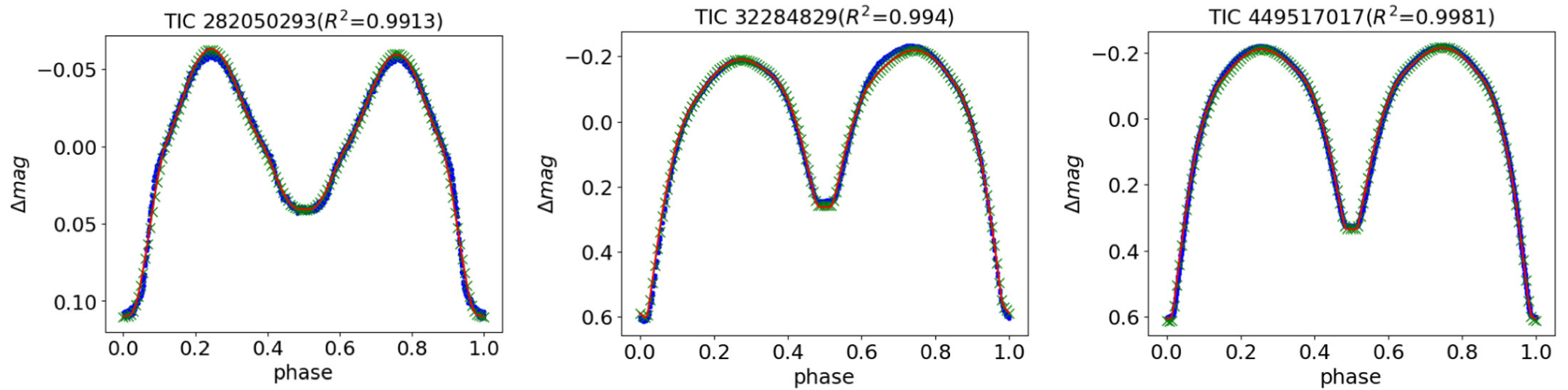
Figure 8. from Xu Ding et al 2025 Astron. J. 169 doi:10.3847/1538-3881/adb846 https://dx.doi.org/10.3847/1538-3881/adb846 © 2025. The Author(s). Published by the American Astronomical Society.
