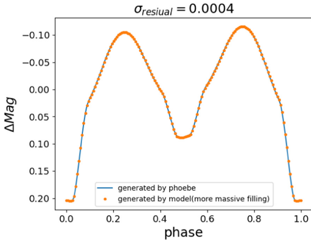
Figure 4. from Xu Ding et al 2025 Astron. J. 169 doi:10.3847/1538-3881/adb846 https://dx.doi.org/10.3847/1538-3881/adb846 © 2025. The Author(s). Published by the American Astronomical Society.
