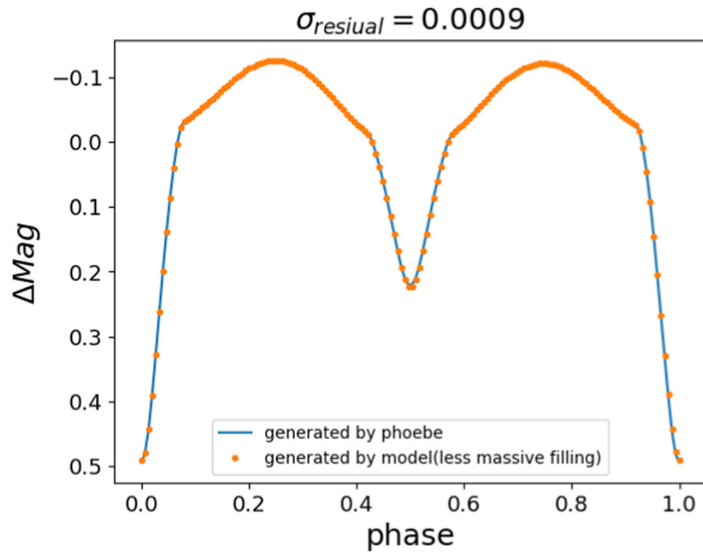
Figure 3. from Xu Ding et al 2025 Astron. J. 169 doi:10.3847/1538-3881/adb846 https://dx.doi.org/10.3847/1538-3881/adb846 © 2025. The Author(s). Published by the American Astronomical Society.
