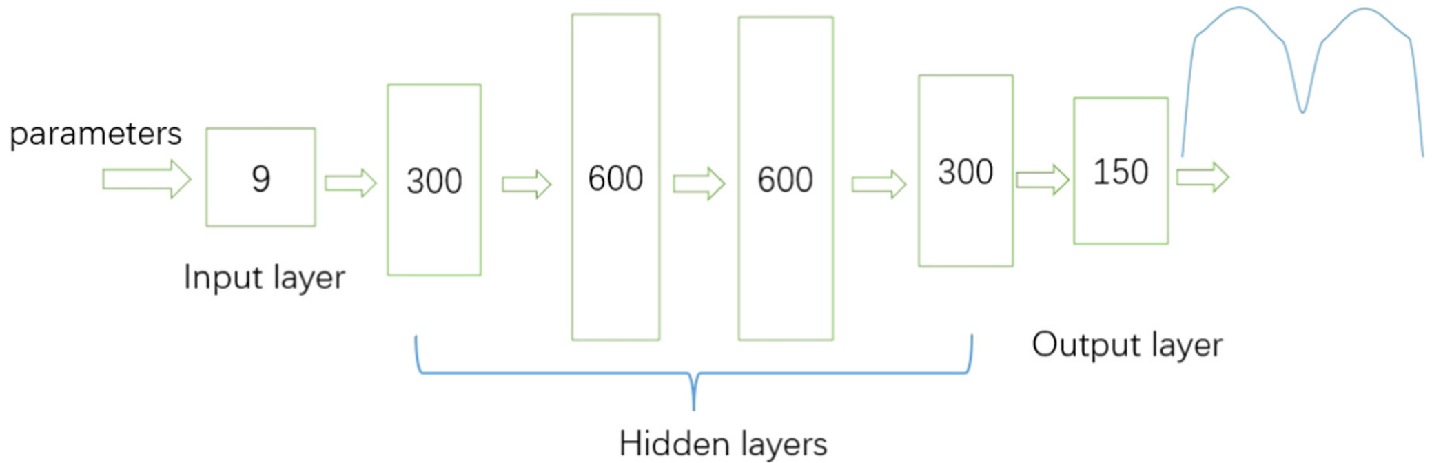
Figure 2. from Xu Ding et al 2025 Astron. J. 169 doi:10.3847/1538-3881/adb846 https://dx.doi.org/10.3847/1538-3881/adb846 © 2025. The Author(s). Published by the American Astronomical Society.
