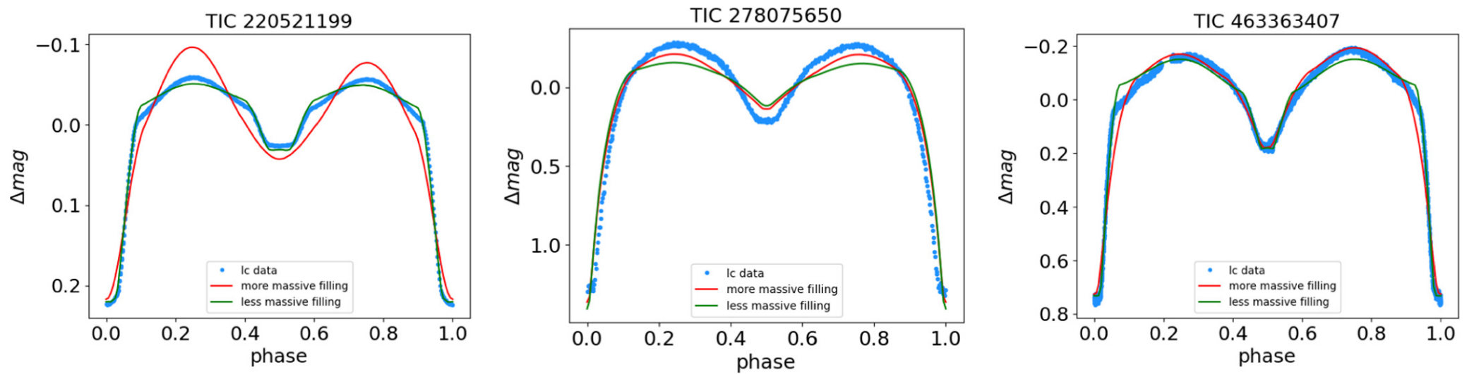
Figure 10. from Xu Ding et al 2025 Astron. J. 169 doi:10.3847/1538-3881/adb846 https://dx.doi.org/10.3847/1538-3881/adb846 © 2025. The Author(s). Published by the American Astronomical Society.
