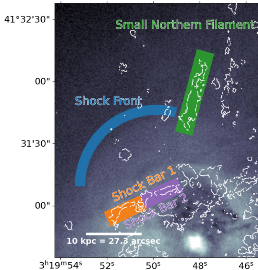
(a) Diagram of the shock region in NGC 1275.
