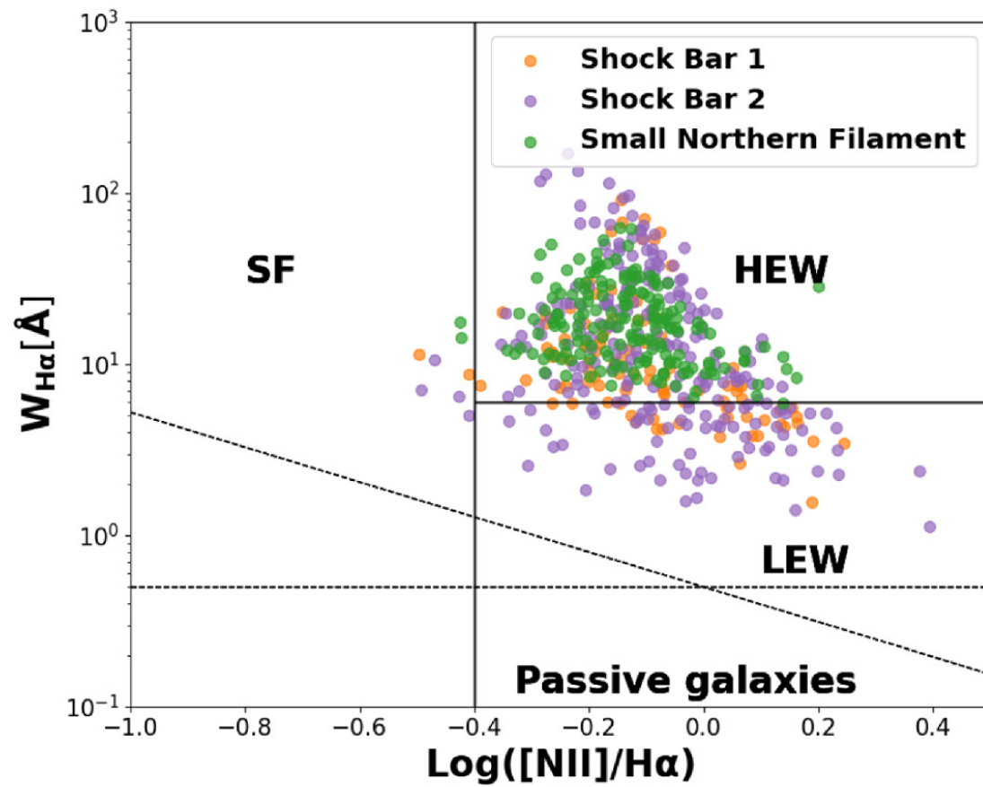
(b) WHAN plot for the bar in the shock region.
