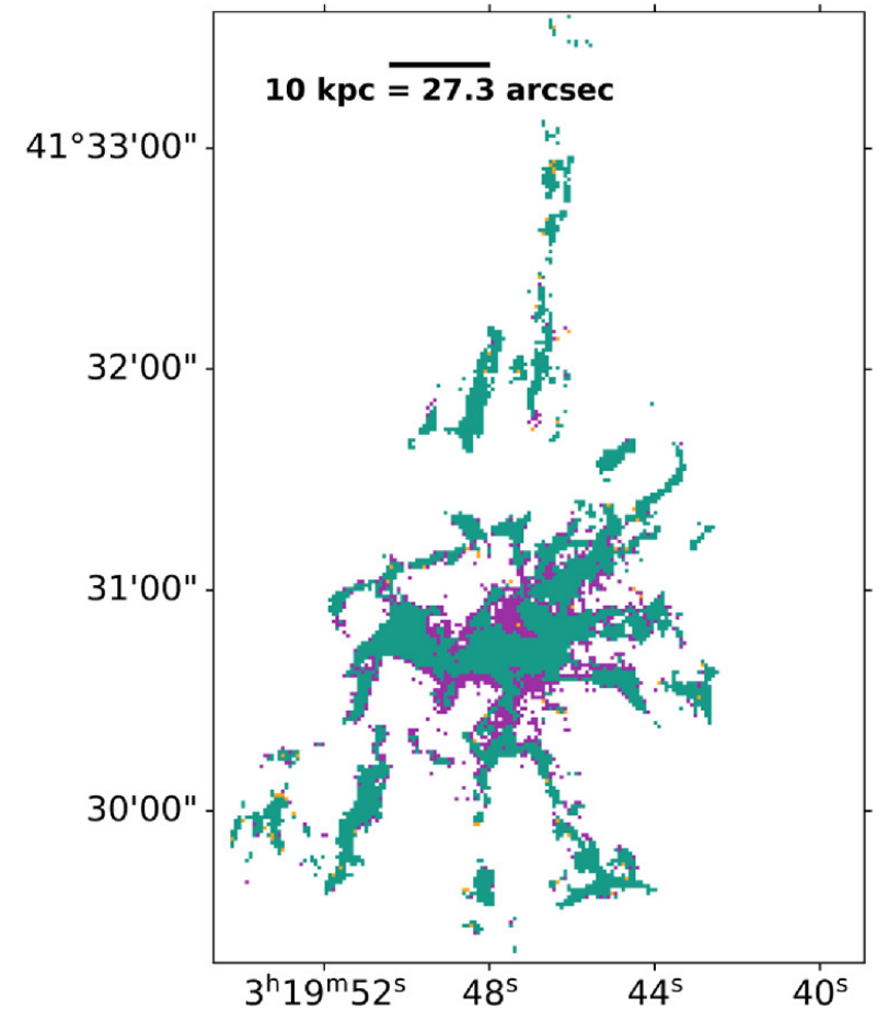
(b) Color-coded emission-line nebula map.
