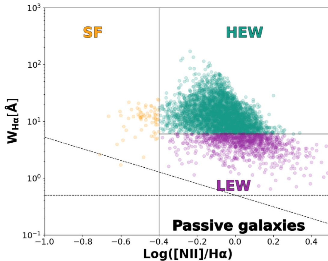
(a) WHAN diagram of emission pixels.
