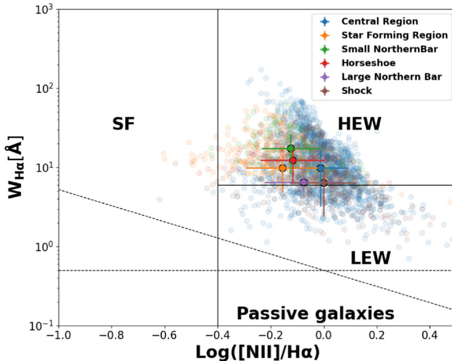
Figure 6. from Carter Lee Rhea et al 2025 Astron. J. 169 doi:10.3847/1538-3881/adb732 https://dx.doi.org/10.3847/1538-3881/adb732 © 2025. The Author(s). Published by the American Astronomical Society.
