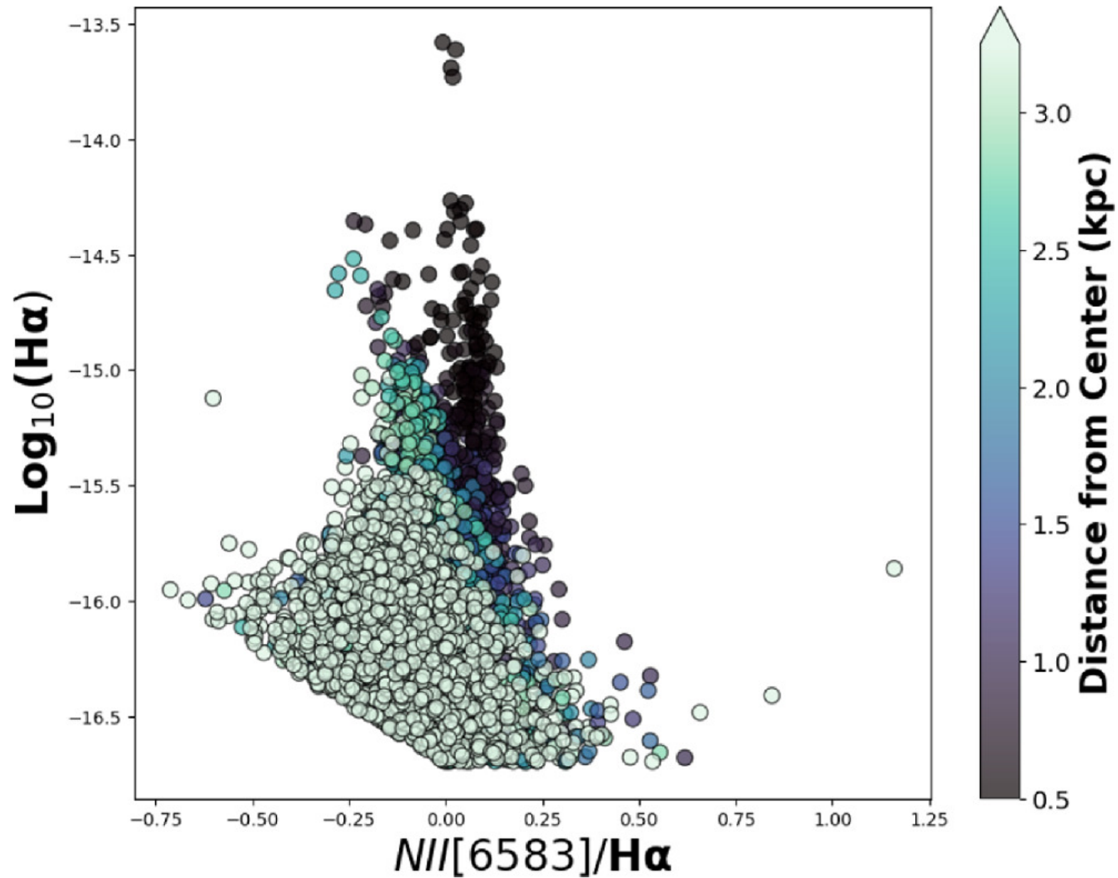
Figure 5. from Carter Lee Rhea et al 2025 Astron. J. 169 doi:10.3847/1538-3881/adb732 https://dx.doi.org/10.3847/1538-3881/adb732 © 2025. The Author(s). Published by the American Astronomical Society.
