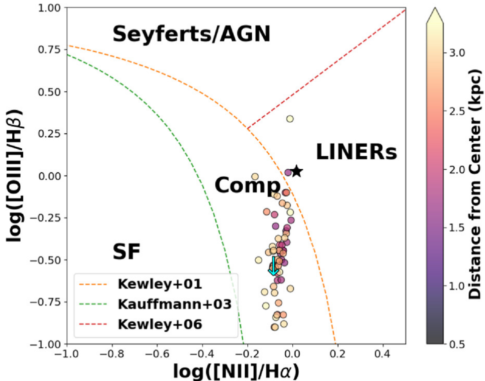
Figure 4. from Carter Lee Rhea et al 2025 Astron. J. 169 doi:10.3847/1538-3881/adb732 https://dx.doi.org/10.3847/1538-3881/adb732 © 2025. The Author(s). Published by the American Astronomical Society.
