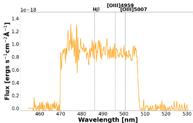
(e) SN2 sky emission
