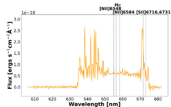
(f) SN3 sky emission
