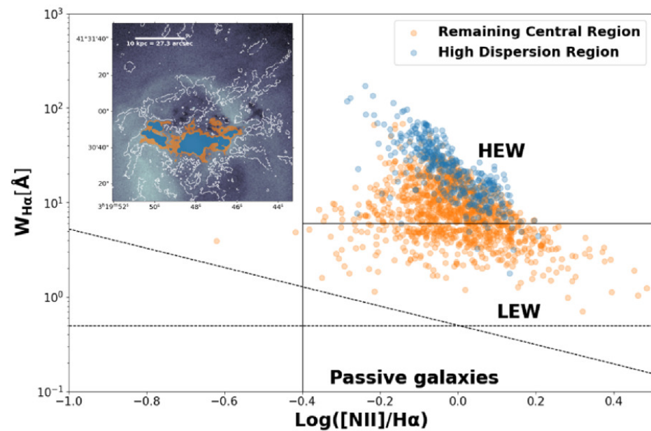
(a) Diagram of the central region of the filamentary nebula.
