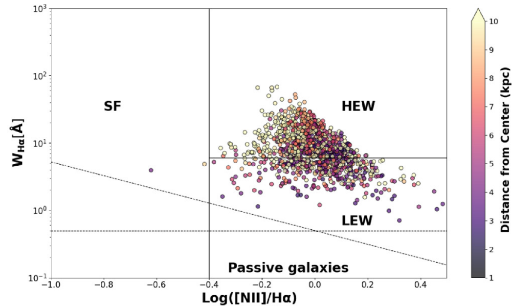
(b) WHAN plot color-coded by distance to the AGN.
