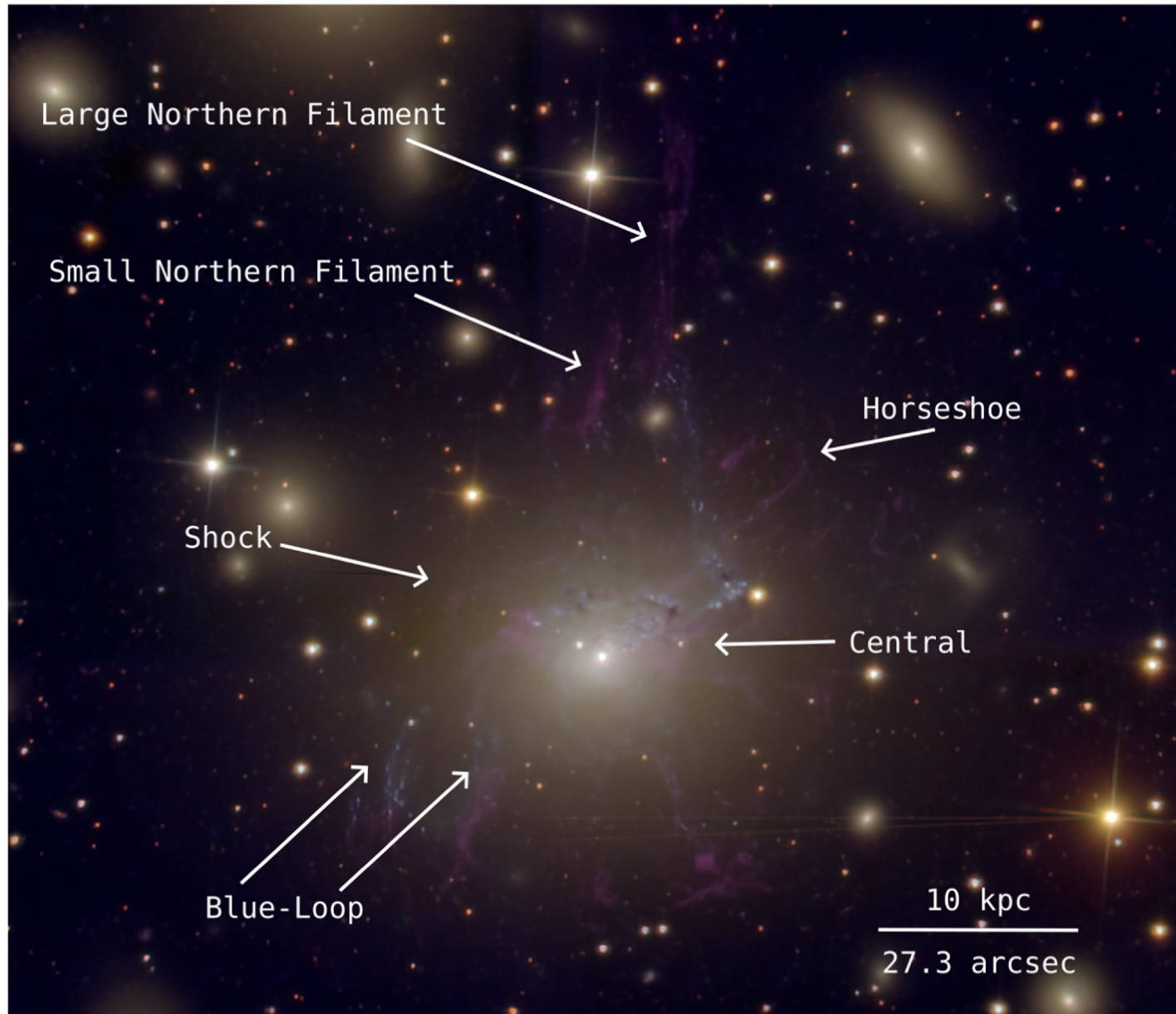
Figure 1. from Carter Lee Rhea et al 2025 Astron. J. 169 doi:10.3847/1538-3881/adb732 https://dx.doi.org/10.3847/1538-3881/adb732 © 2025. The Author(s). Published by the American Astronomical Society.
