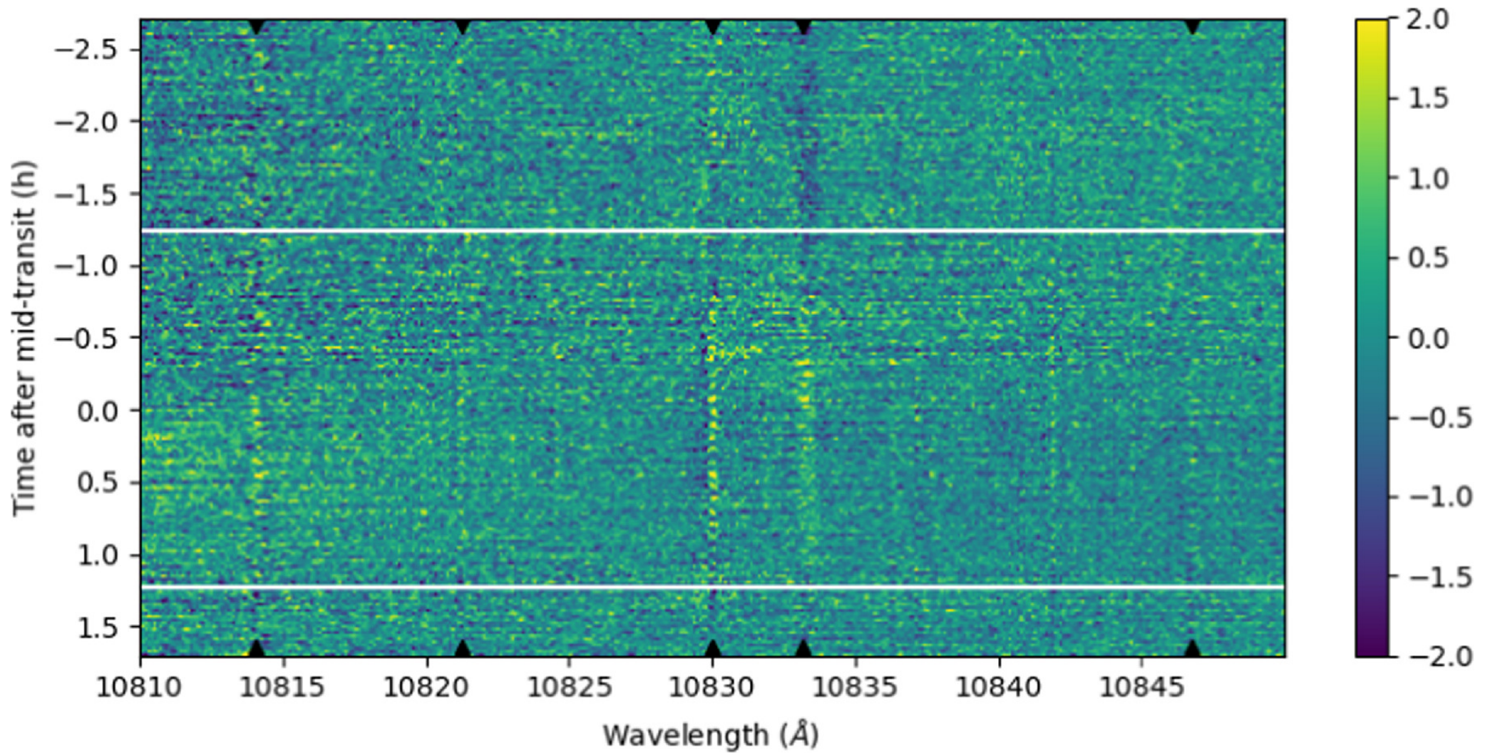
Figure 9. from Michael Zhang et al 2025 Astron. J. 169 doi:10.3847/1538-3881/adb490 https://dx.doi.org/10.3847/1538-3881/adb490 © 2025. The Author(s). Published by the American Astronomical Society.
