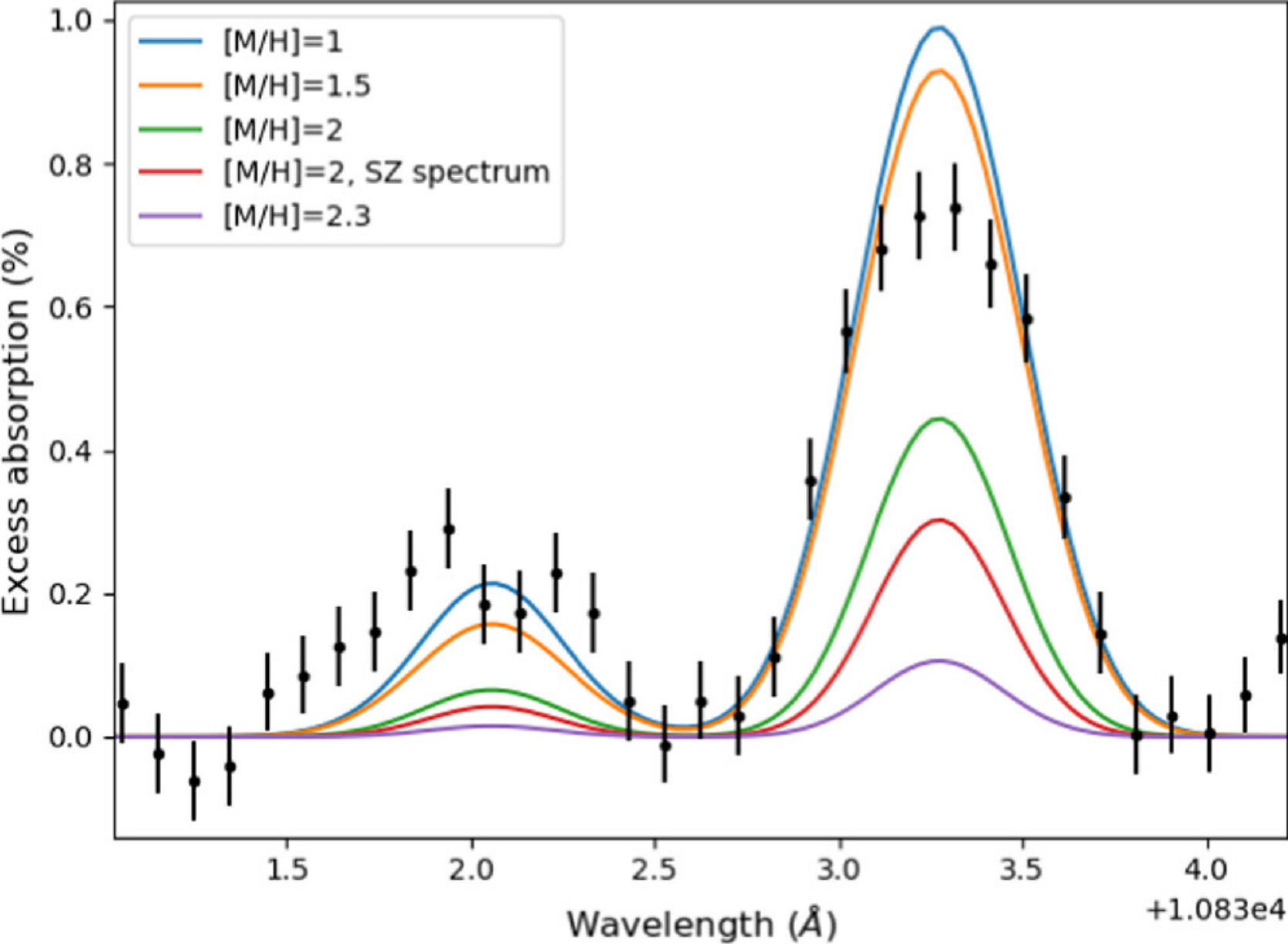
Figure 7. from Michael Zhang et al 2025 Astron. J. 169 doi:10.3847/1538-3881/adb490 https://dx.doi.org/10.3847/1538-3881/adb490 © 2025. The Author(s). Published by the American Astronomical Society.
