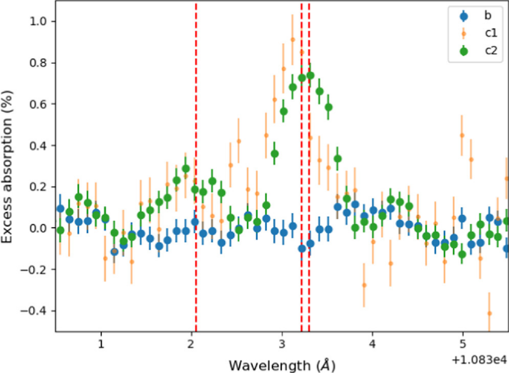
Figure 4. from Michael Zhang et al 2025 Astron. J. 169 doi:10.3847/1538-3881/adb490 https://dx.doi.org/10.3847/1538-3881/adb490 © 2025. The Author(s). Published by the American Astronomical Society.
