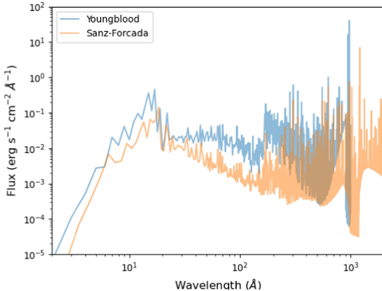
Figure 2. from Michael Zhang et al 2025 Astron. J. 169 doi:10.3847/1538-3881/adb490 https://dx.doi.org/10.3847/1538-3881/adb490 © 2025. The Author(s). Published by the American Astronomical Society.
