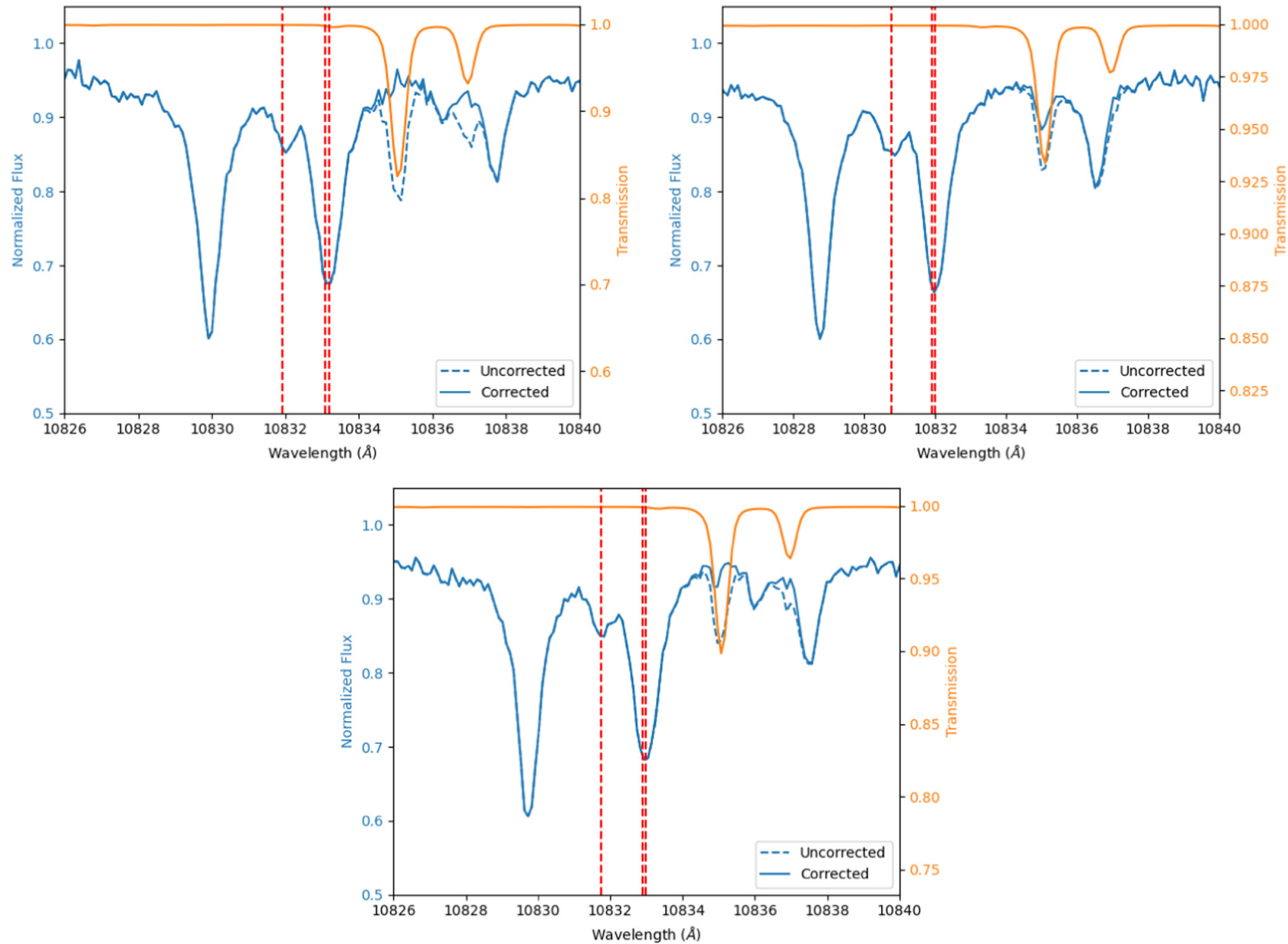
Figure 11. from Michael Zhang et al 2025 Astron. J. 169 doi:10.3847/1538-3881/adb490 https://dx.doi.org/10.3847/1538-3881/adb490 © 2025. The Author(s). Published by the American Astronomical Society.
