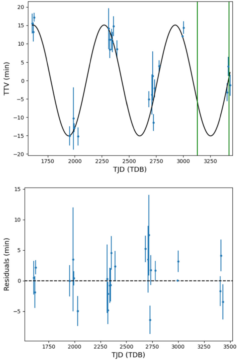
Figure 1. from Michael Zhang et al 2025 Astron. J. 169 doi:10.3847/1538-3881/adb490 https://dx.doi.org/10.3847/1538-3881/adb490 © 2025. The Author(s). Published by the American Astronomical Society.
