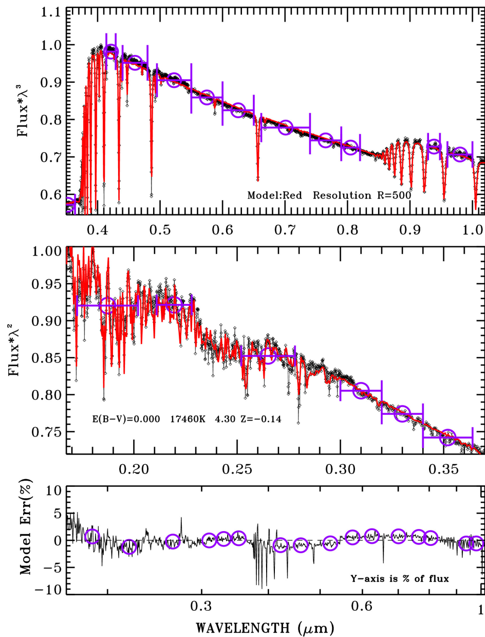
Figure 3. from Ivan Hubeny et al 2025 Astron. J. 169 doi:10.3847/1538-3881/adb1bf https://dx.doi.org/10.3847/1538-3881/adb1bf © 2025. The Author(s). Published by the American Astronomical Society.
