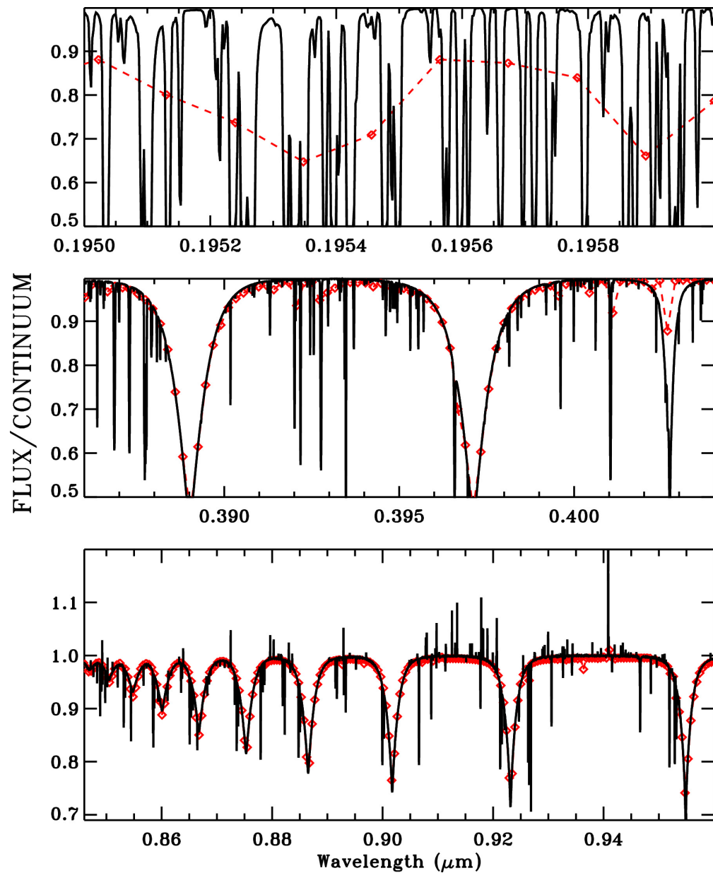
Figure 2. from Ivan Hubeny et al 2025 Astron. J. 169 doi:10.3847/1538-3881/adb1bf https://dx.doi.org/10.3847/1538-3881/adb1bf © 2025. The Author(s). Published by the American Astronomical Society.
