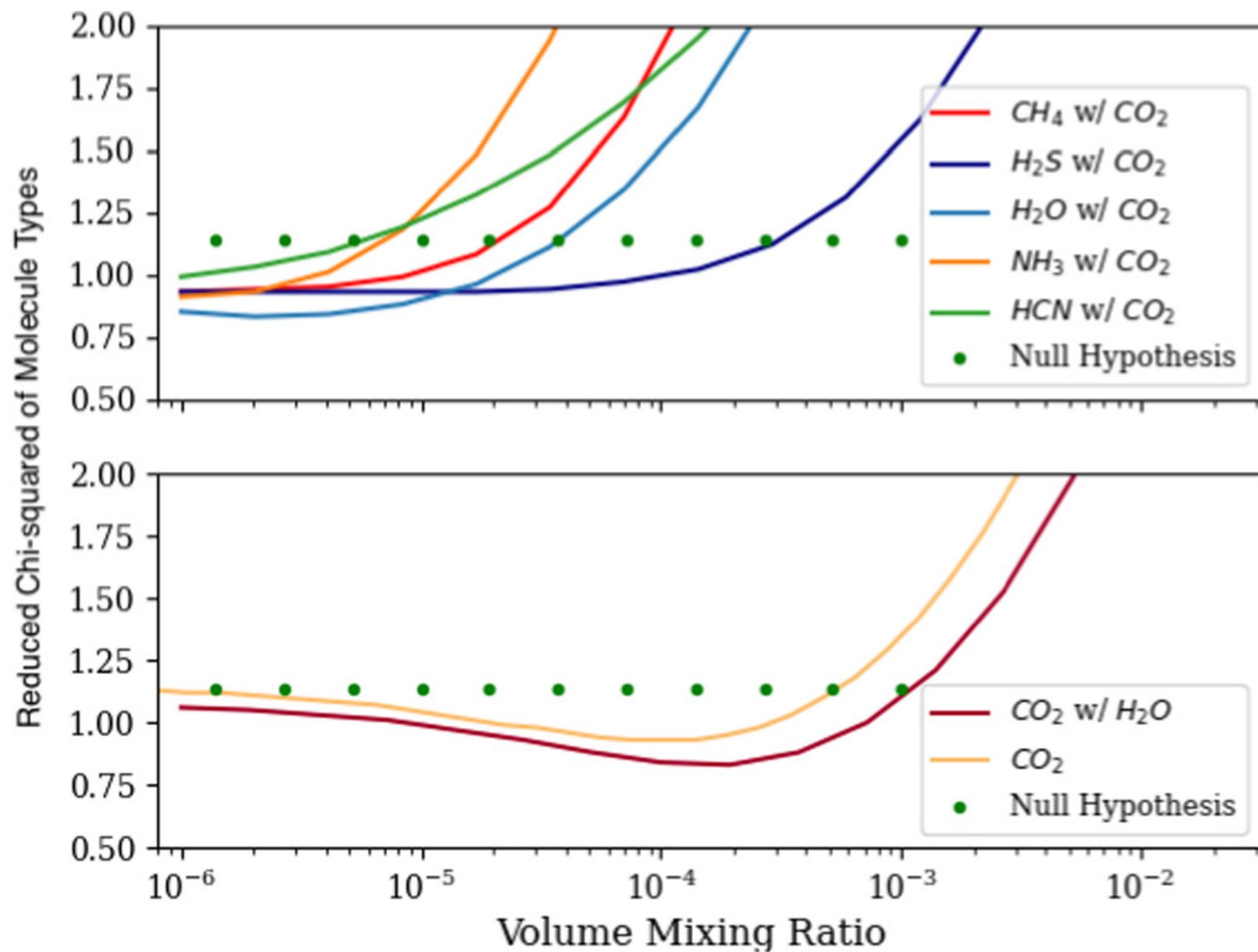
Figure 9. from Thomas Barclay et al 2025 Astron. J. 169 doi:10.3847/1538-3881/ada5f6 https://dx.doi.org/10.3847/1538-3881/ada5f6 © 2025. The Author(s). Published by the American Astronomical Society.
