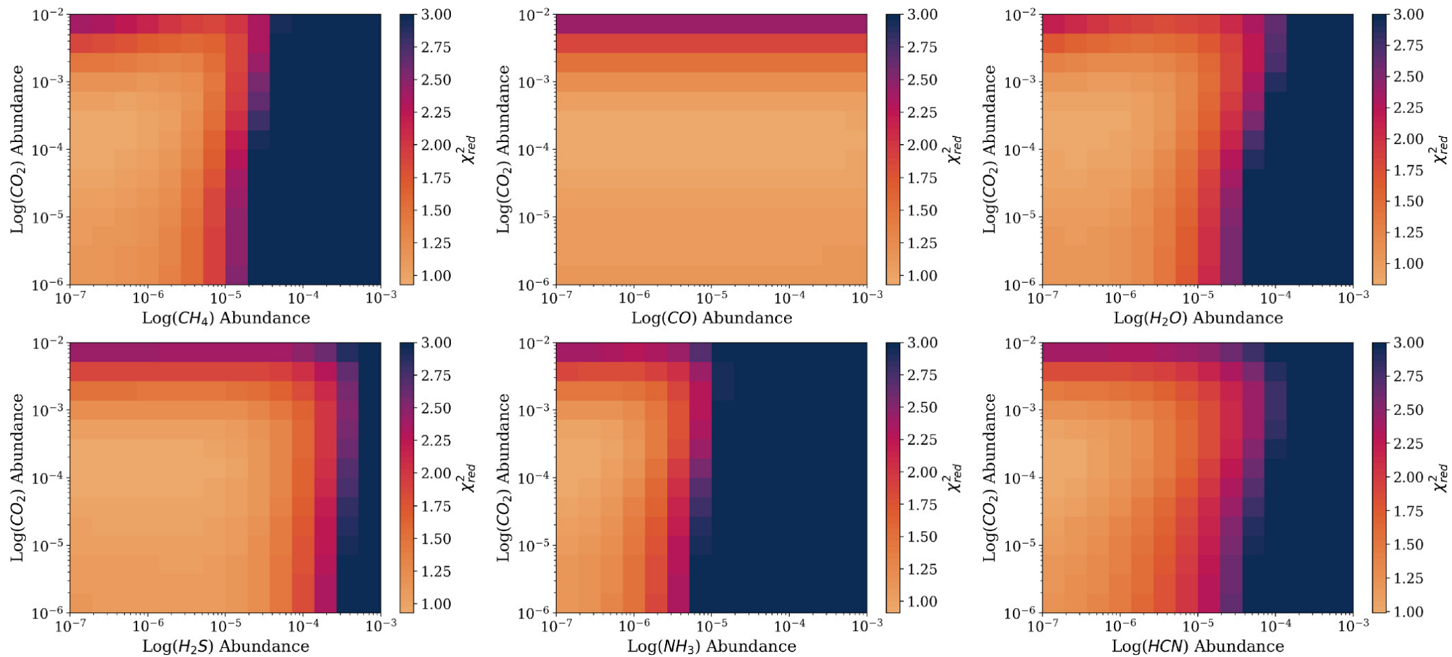
Figure 8. from Thomas Barclay et al 2025 Astron. J. 169 doi:10.3847/1538-3881/ada5f6 https://dx.doi.org/10.3847/1538-3881/ada5f6 © 2025. The Author(s). Published by the American Astronomical Society.
