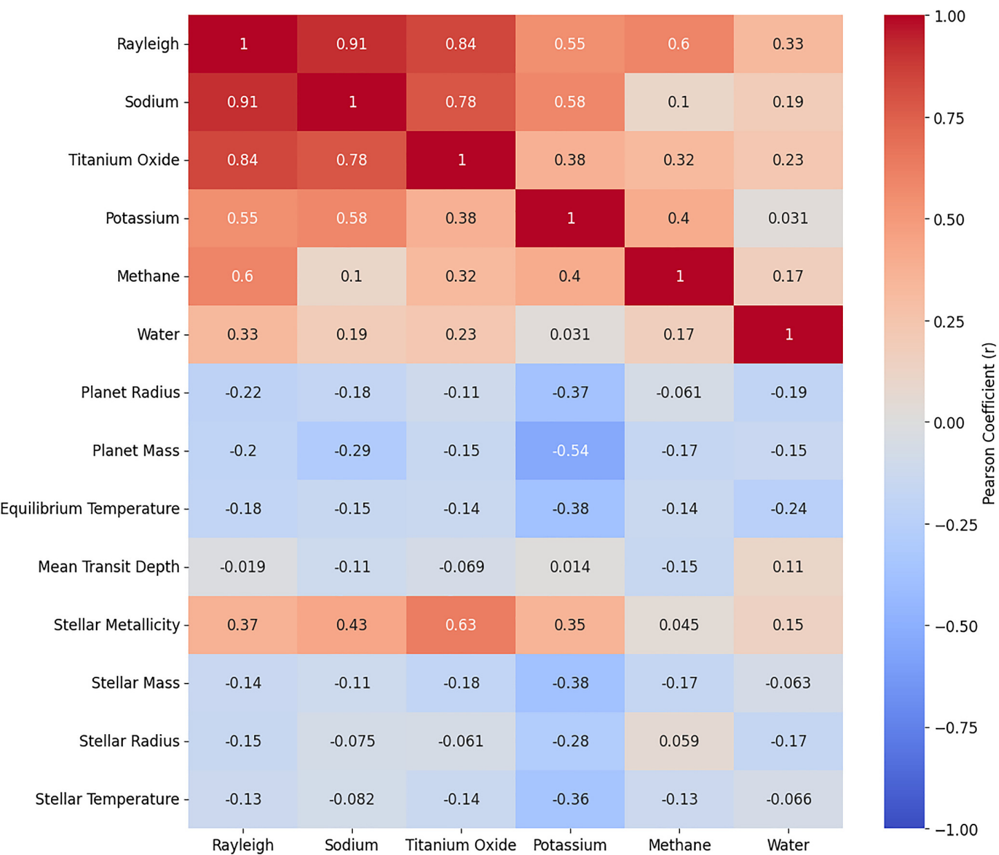
Figure 8. from Ryan J. Oelkers et al 2025 Astron. J. 169 doi:10.3847/1538-3881/ada557 https://dx.doi.org/10.3847/1538-3881/ada557 © 2025. The Author(s). Published by the American Astronomical Society.
