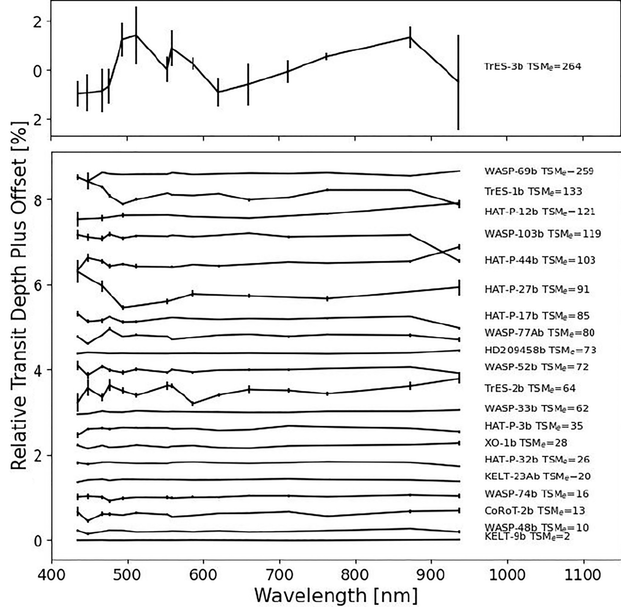
Figure 7. from Ryan J. Oelkers et al 2025 Astron. J. 169 doi:10.3847/1538-3881/ada557 https://dx.doi.org/10.3847/1538-3881/ada557 © 2025. The Author(s). Published by the American Astronomical Society.
