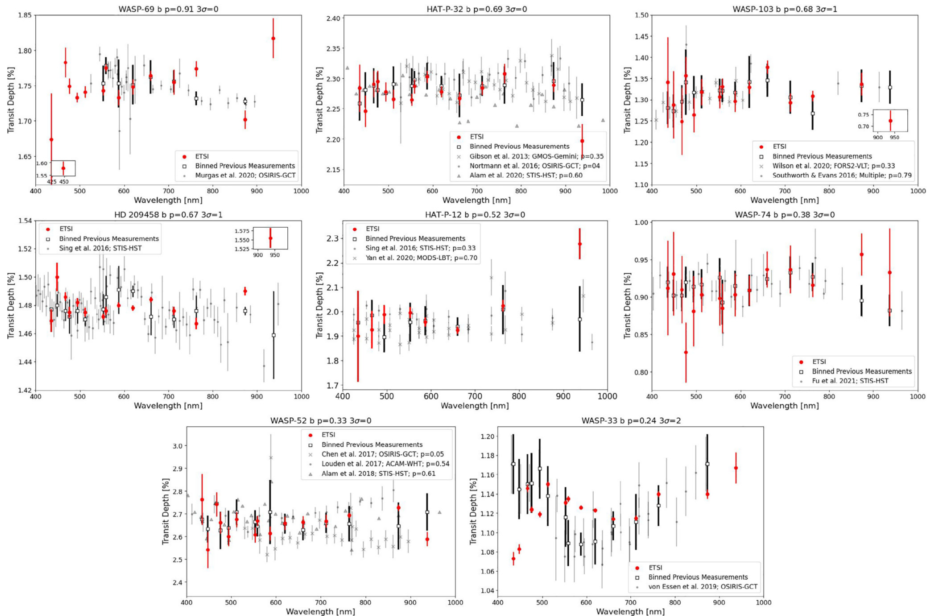
Figure 6. from Ryan J. Oelkers et al 2025 Astron. J. 169 doi:10.3847/1538-3881/ada557 https://dx.doi.org/10.3847/1538-3881/ada557 © 2025. The Author(s). Published by the American Astronomical Society.
