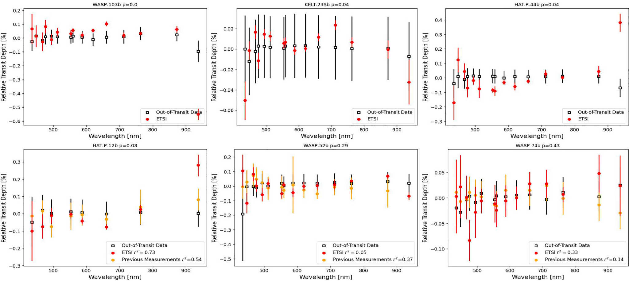
Figure 5. from Ryan J. Oelkers et al 2025 Astron. J. 169 doi:10.3847/1538-3881/ada557 https://dx.doi.org/10.3847/1538-3881/ada557 © 2025. The Author(s). Published by the American Astronomical Society.
