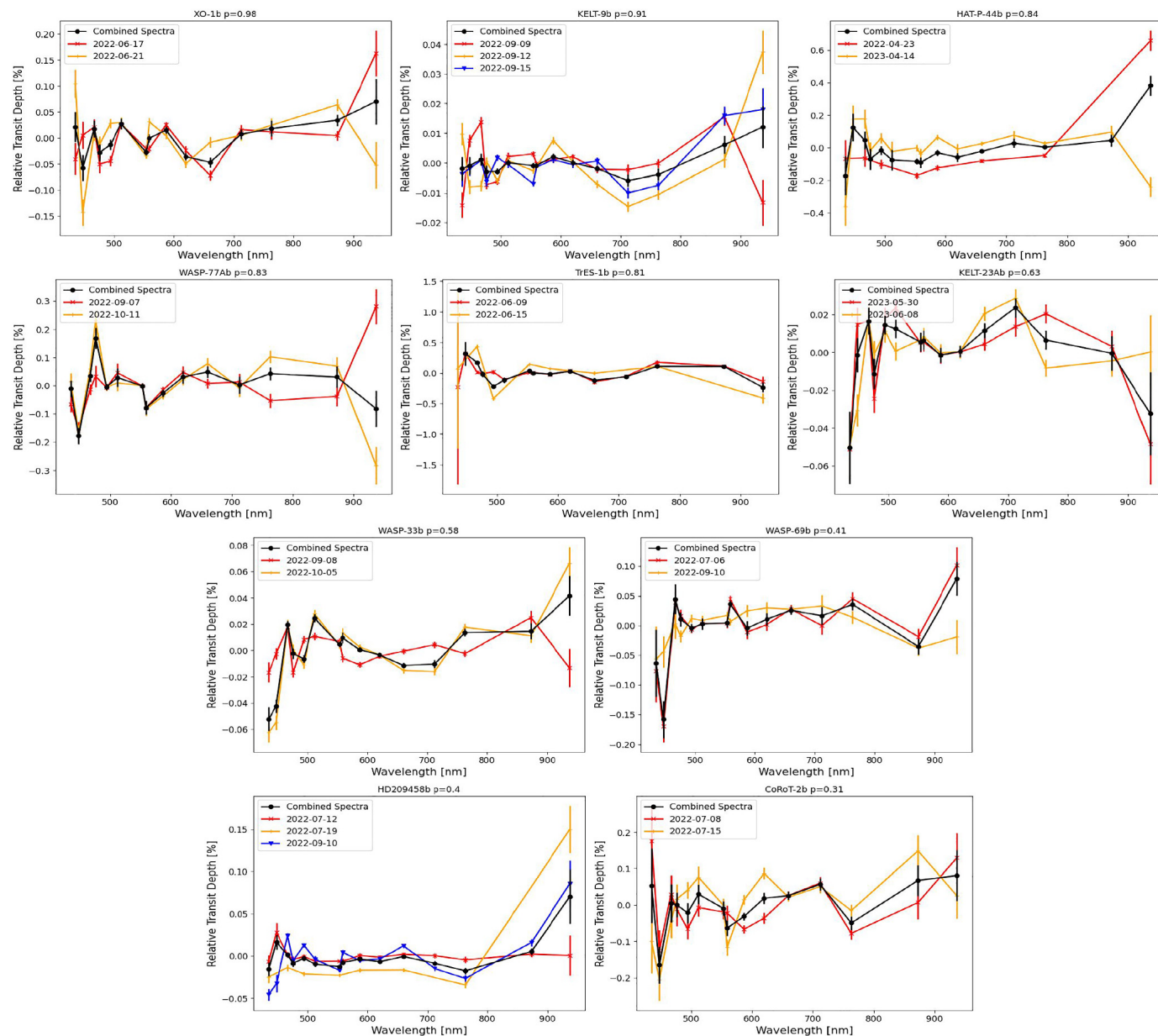
Figure 4. from Ryan J. Oelkers et al 2025 Astron. J. 169 doi:10.3847/1538-3881/ada557 https://dx.doi.org/10.3847/1538-3881/ada557 © 2025. The Author(s). Published by the American Astronomical Society.
