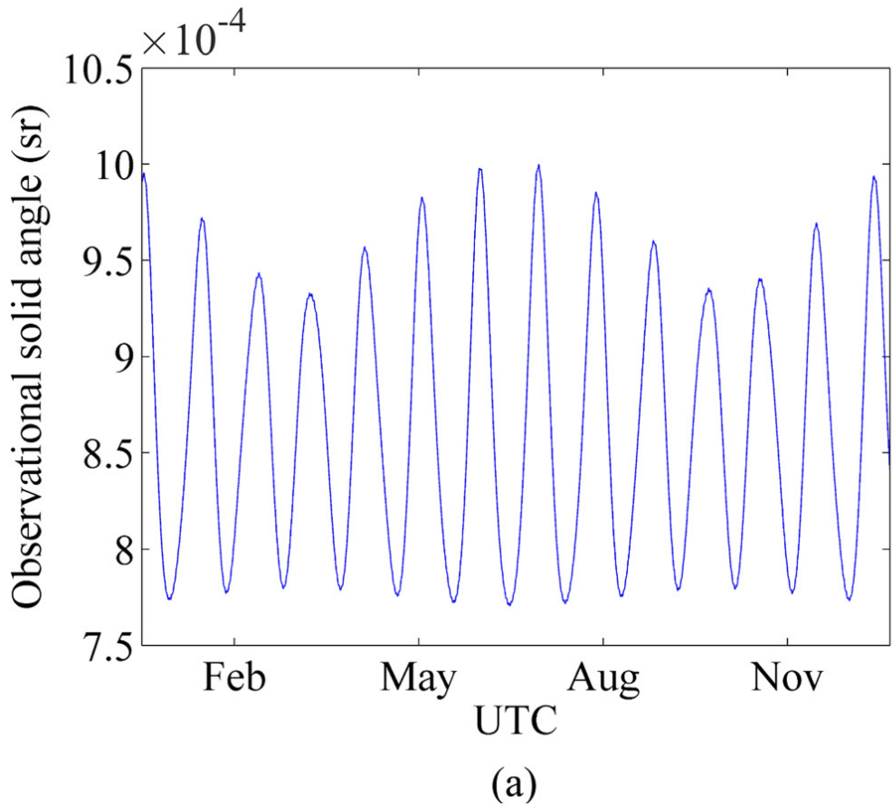
Figure 2. from Hanlin Ye et al 2025 Astron. J. 169 doi:10.3847/1538-3881/ada4b4 https://dx.doi.org/10.3847/1538-3881/ada4b4 © 2025. The Author(s). Published by the American Astronomical Society.
