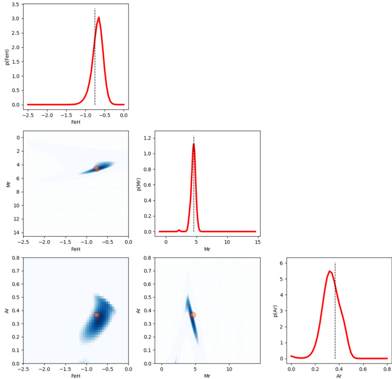
Figure 9. from Lovro Palaversa et al 2025 Astron. J. 169 doi:10.3847/1538-3881/ada3c2 https://dx.doi.org/10.3847/1538-3881/ada3c2 © 2025. The Author(s). Published by the American Astronomical Society.
