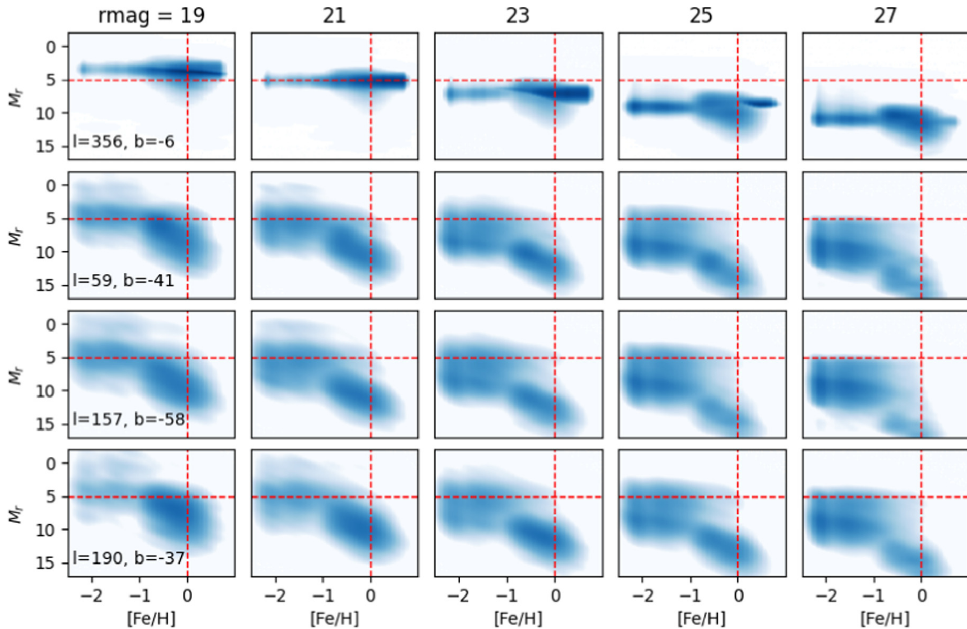
Figure 7. from Lovro Palaversa et al 2025 Astron. J. 169 doi:10.3847/1538-3881/ada3c2 https://dx.doi.org/10.3847/1538-3881/ada3c2 © 2025. The Author(s). Published by the American Astronomical Society.
