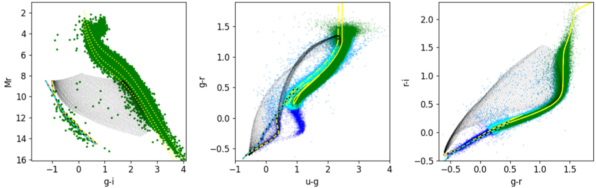
Figure 6. from Lovro Palaversa et al 2025 Astron. J. 169 doi:10.3847/1538-3881/ada3c2 https://dx.doi.org/10.3847/1538-3881/ada3c2 © 2025. The Author(s). Published by the American Astronomical Society.
