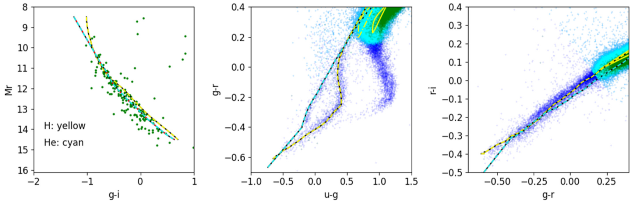
Figure 5. from Lovro Palaversa et al 2025 Astron. J. 169 doi:10.3847/1538-3881/ada3c2 https://dx.doi.org/10.3847/1538-3881/ada3c2 © 2025. The Author(s). Published by the American Astronomical Society.
