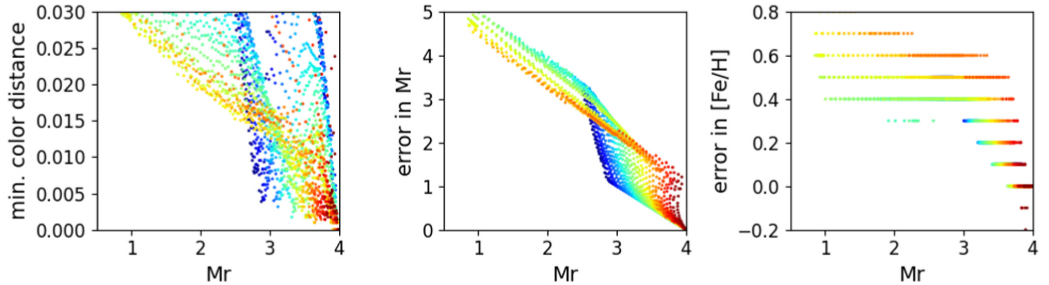
Figure 4. from Lovro Palaversa et al 2025 Astron. J. 169 doi:10.3847/1538-3881/ada3c2 https://dx.doi.org/10.3847/1538-3881/ada3c2 © 2025. The Author(s). Published by the American Astronomical Society.
