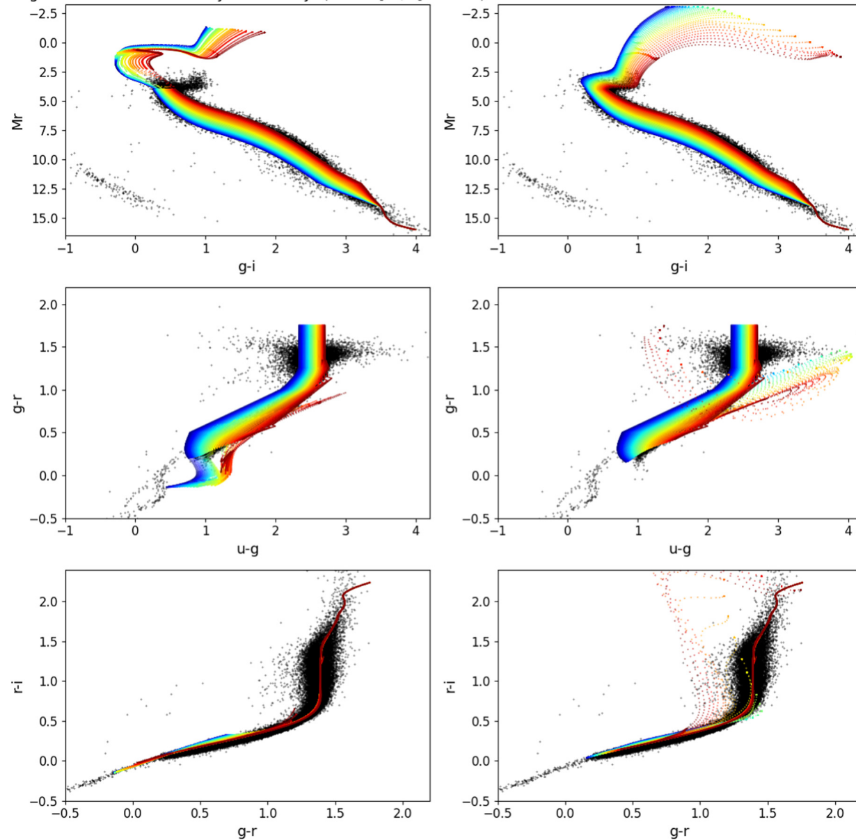
Figure 3. from Lovro Palaversa et al 2025 Astron. J. 169 doi:10.3847/1538-3881/ada3c2 https://dx.doi.org/10.3847/1538-3881/ada3c2 © 2025. The Author(s). Published by the American Astronomical Society.
