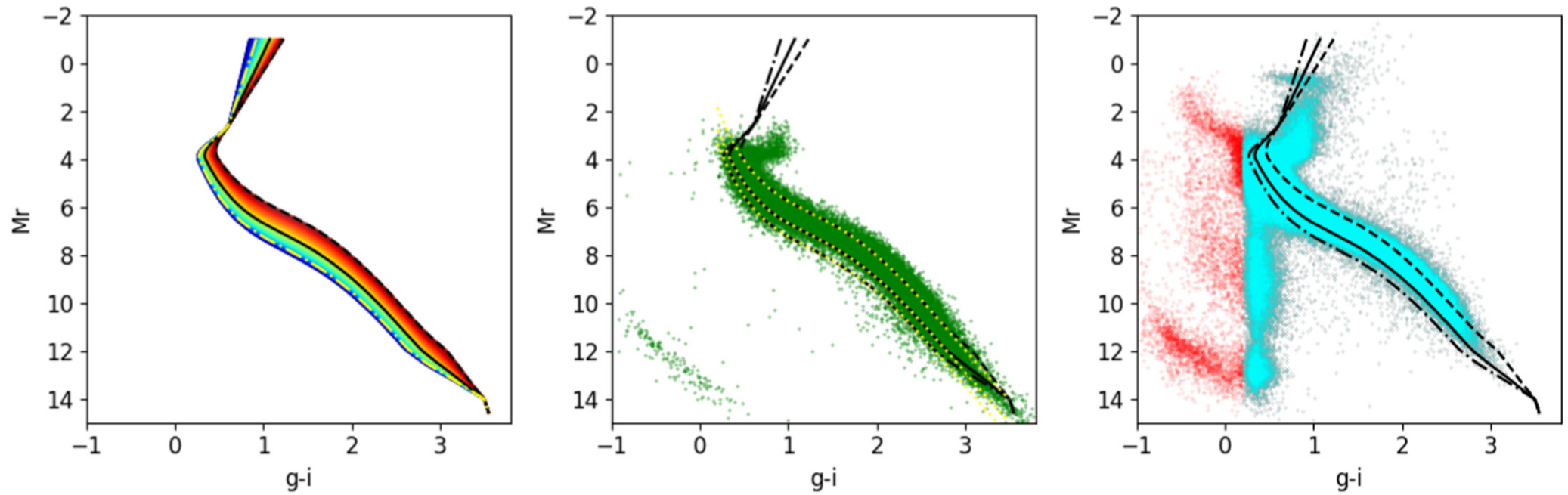
Figure 2. from Lovro Palaversa et al 2025 Astron. J. 169 doi:10.3847/1538-3881/ada3c2 https://dx.doi.org/10.3847/1538-3881/ada3c2 © 2025. The Author(s). Published by the American Astronomical Society.
