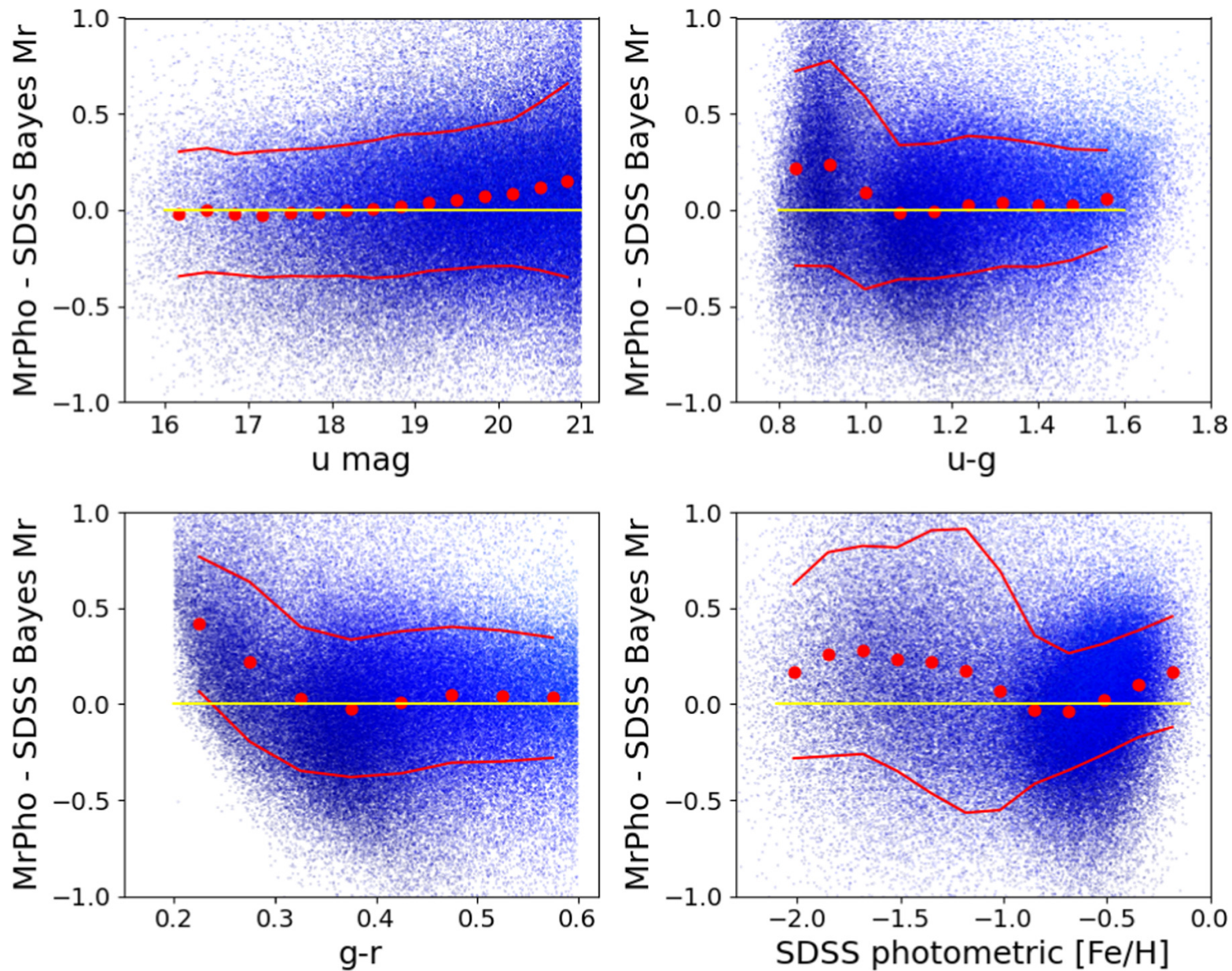
Figure 16. from Lovro Palaversa et al 2025 Astron. J. 169 doi:10.3847/1538-3881/ada3c2 https://dx.doi.org/10.3847/1538-3881/ada3c2 © 2025. The Author(s). Published by the American Astronomical Society.
