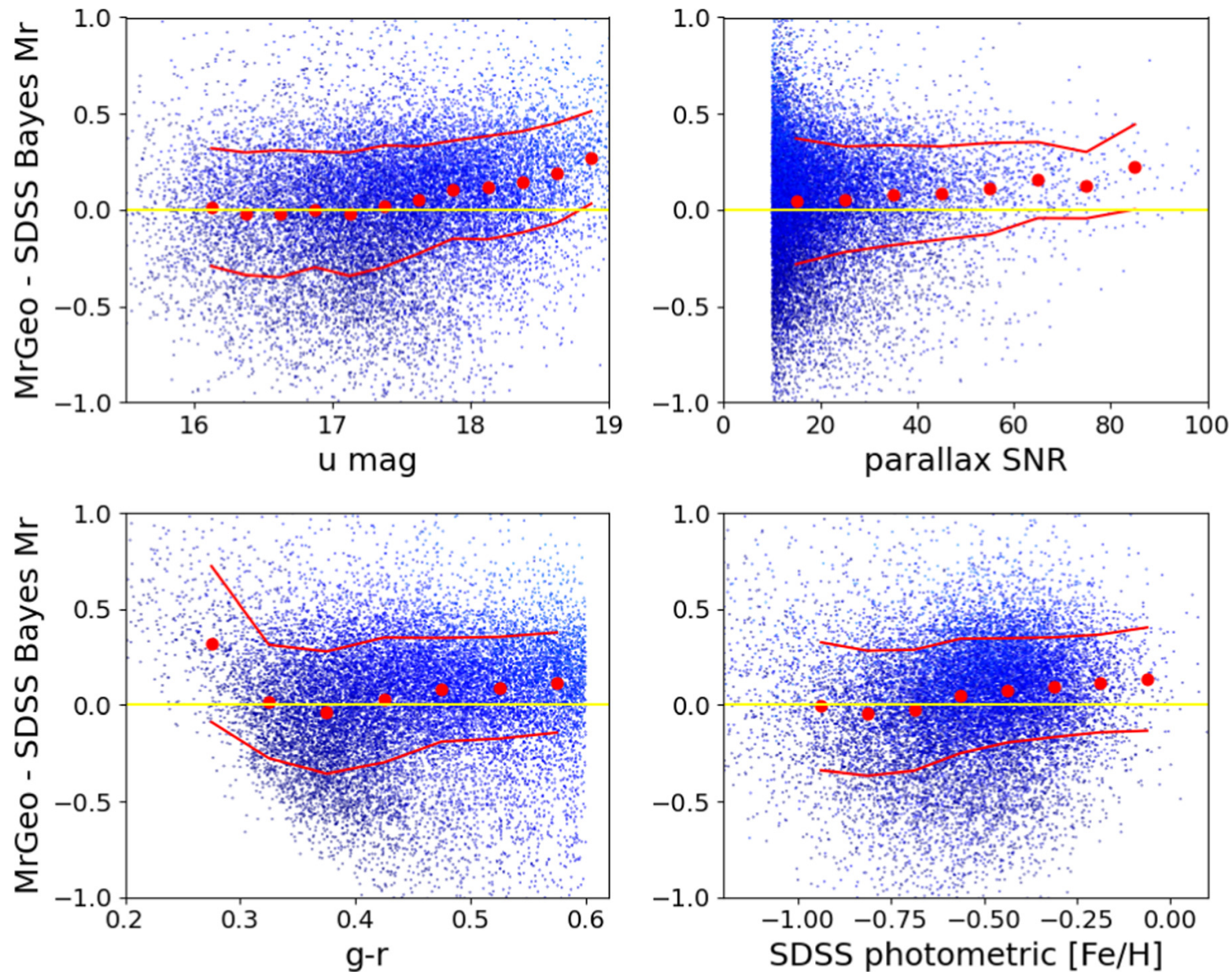
Figure 15. from Lovro Palaversa et al 2025 Astron. J. 169 doi:10.3847/1538-3881/ada3c2 https://dx.doi.org/10.3847/1538-3881/ada3c2 © 2025. The Author(s). Published by the American Astronomical Society.
