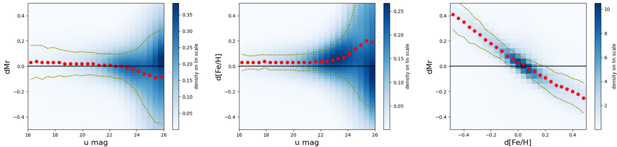
Figure 14. from Lovro Palaversa et al 2025 Astron. J. 169 doi:10.3847/1538-3881/ada3c2 https://dx.doi.org/10.3847/1538-3881/ada3c2 © 2025. The Author(s). Published by the American Astronomical Society.
