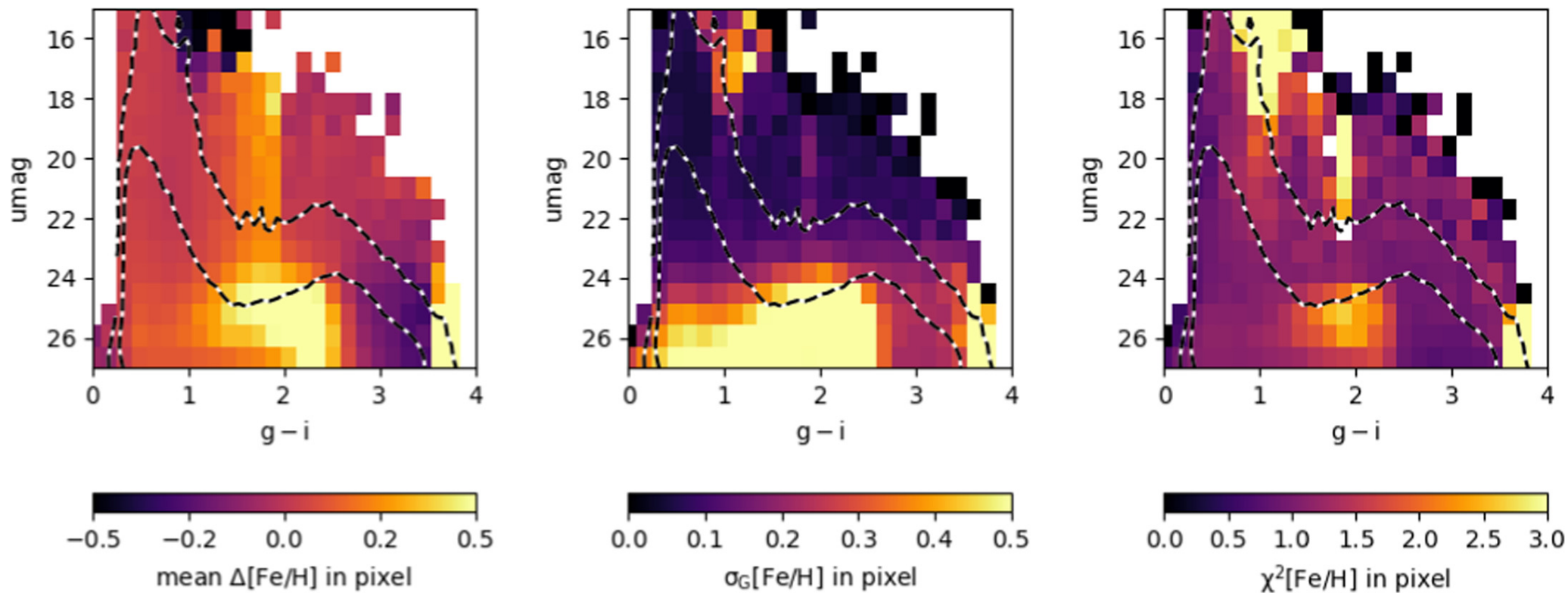
Figure 13. from Lovro Palaversa et al 2025 Astron. J. 169 doi:10.3847/1538-3881/ada3c2 https://dx.doi.org/10.3847/1538-3881/ada3c2 © 2025. The Author(s). Published by the American Astronomical Society.
