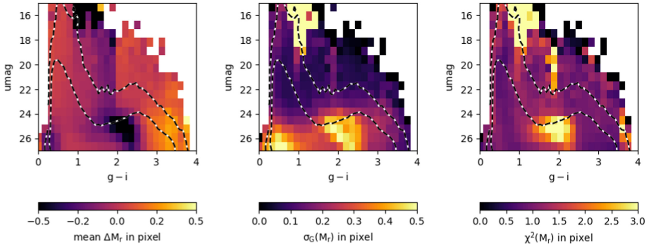
Figure 12. from Lovro Palaversa et al 2025 Astron. J. 169 doi:10.3847/1538-3881/ada3c2 https://dx.doi.org/10.3847/1538-3881/ada3c2 © 2025. The Author(s). Published by the American Astronomical Society.
